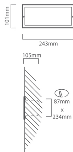
O355 CAD DIAGRAM
