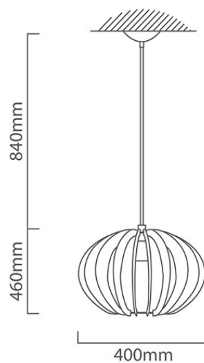
P143 CAD DIAGRAM
