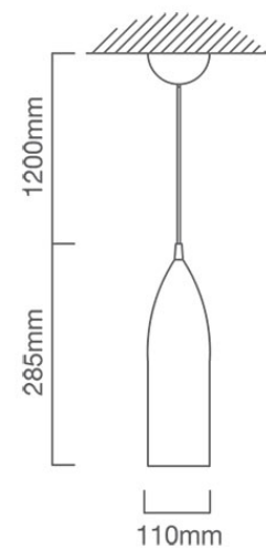
P151 CAD DIAGRAM
