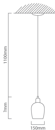
P180 CAD DIAGRAM
