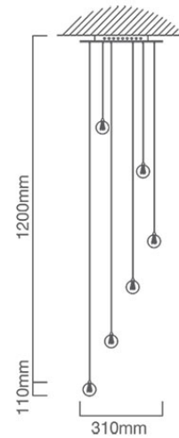
P255 CAD DIAGRAM
