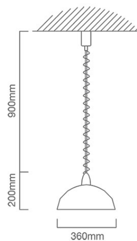
P289 CAD DIAGRAM
