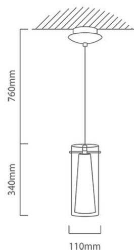
P389 CAD DIAGRAM
