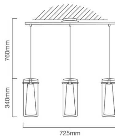
P390 CAD DIAGRAM
