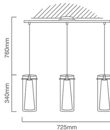
P399 CAD DIAGRAM
