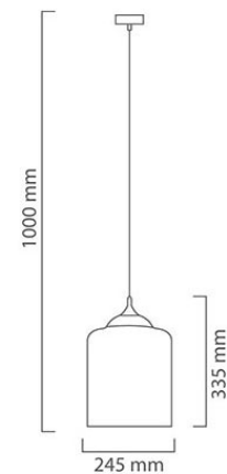
P424 CAD DIAGRAM
