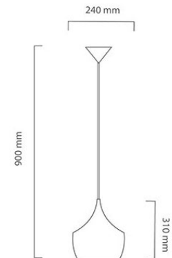
P444 CAD DIAGRAM
