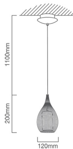
P465 CAD DIAGRAM
