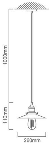
P472 CAD DIAGRAM
