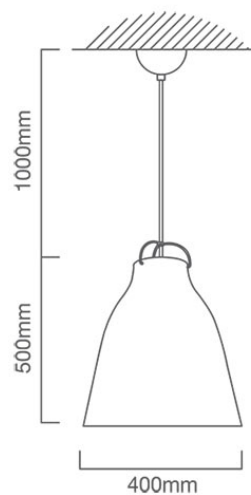
P475 CAD DIAGRAM
