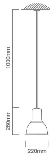
P476 CAD DIAGRAM
