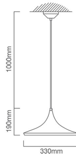
P480BG CAD DIAGRAM
