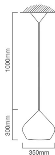
P481 CAD DIAGRAM
