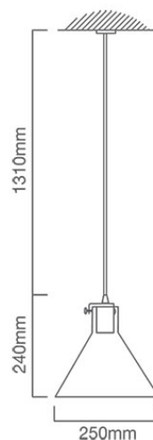
P482 CAD DIAGRAM
