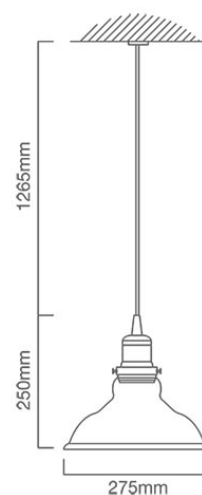
P485 CAD DIAGRAM
