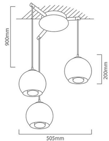
P500 CAD DIAGRAM
