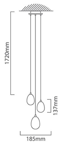
P561 CAD DIAGRAM
