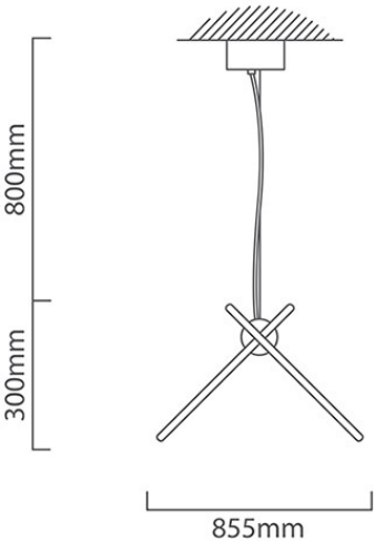
P574 CAD DIAGRAM
