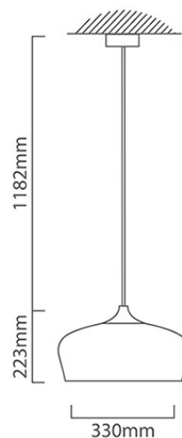
P581 CAD DIAGRAM
