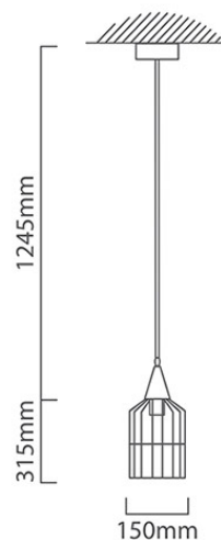
P597 CAD DIAGRAM
