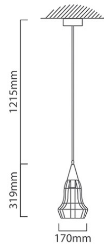
P598 CAD DIAGRAM
