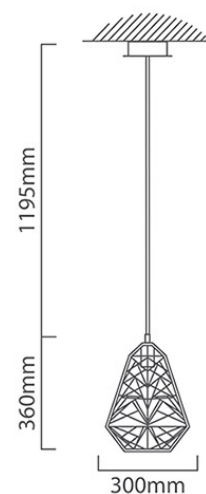
P600 CAD DIAGRAM
