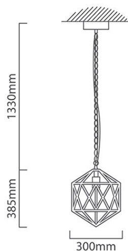
P607 CAD DIAGRAM
