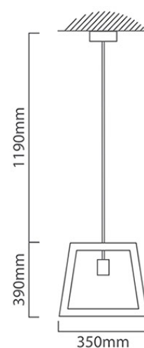
P608 CAD DIAGRAM
