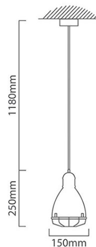
P609 CAD DIAGRAM
