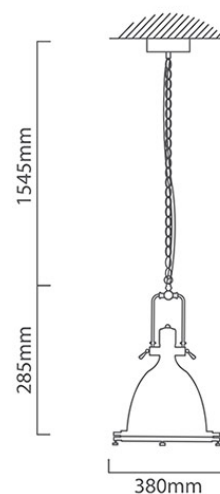
P612 CAD DIAGRAM
