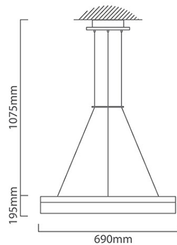
P616 CAD DIAGRAM
