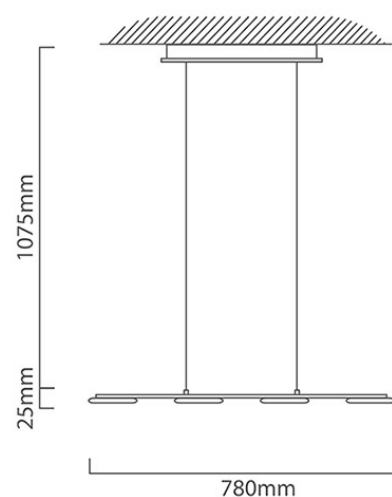
P667 CAD DIAGRAM
