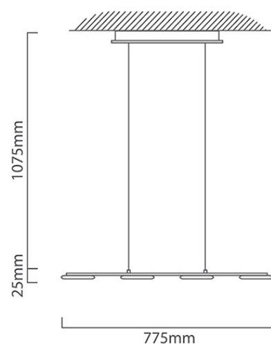
P668 CAD DIAGRAM
