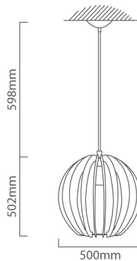
P671M CAD DIAGRAM
