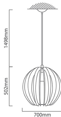
P672 CAD DIAGRAM
