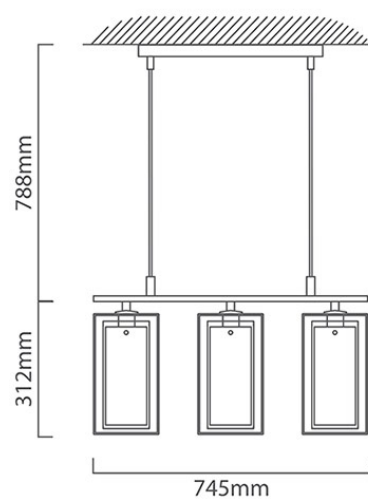
P681 CAD DIAGRAM
