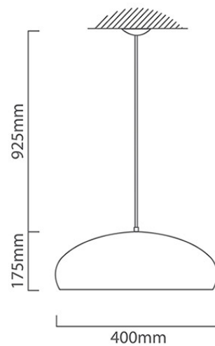
P685 CAD DIAGRAM
