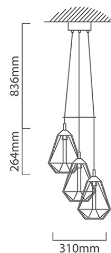
P691 CAD DIAGRAM
