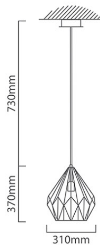
P704 CAD DIAGRAM
