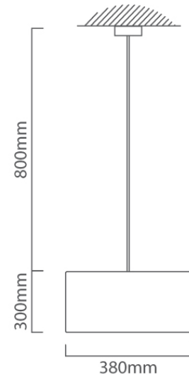
P711B CAD DIAGRAM
