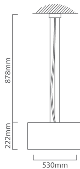
P712 CAD DIAGRAM
