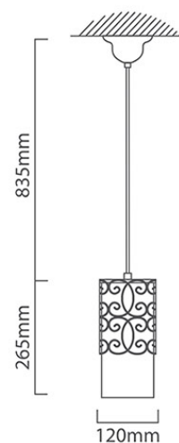
P717 CAD DIAGRAM
