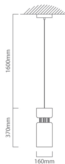
P752 CAD DIAGRAM
