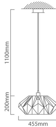
P778B CAD DIAGRAM
