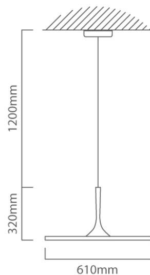
P803 CAD DIAGRAM
