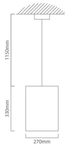
P807 CAD DIAGRAM
