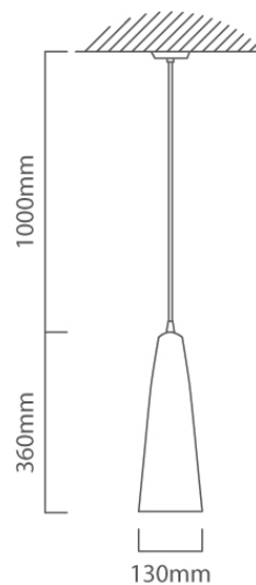
P894 CAD DIAGRAM
