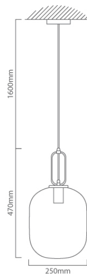
P899CL CAD DIAGRAM
