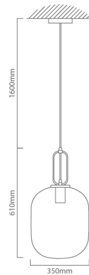
P900CL CAD DIAGRAM
