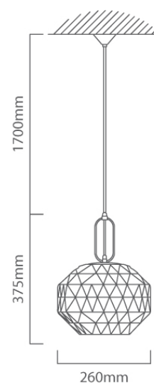
P903 CAD DIAGRAM
